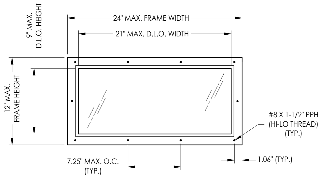
"Spotlights" Lite Frame System 24.0" X 12.0"
