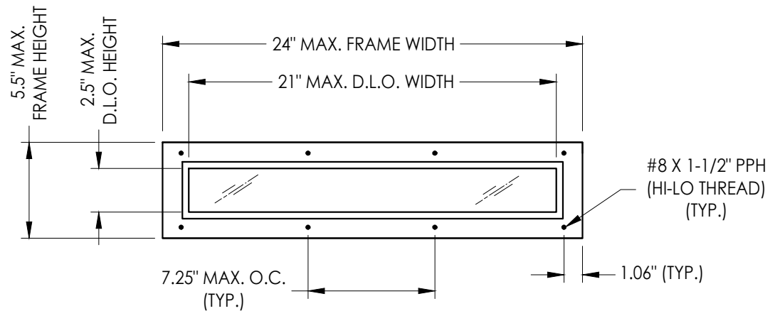
"Spotlights" Lite Frame System 24.0" X 5.5"
